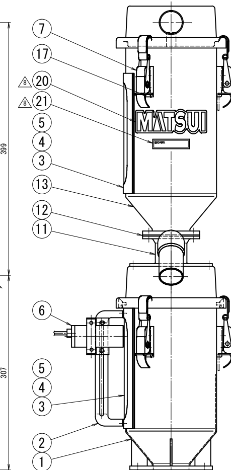
In case of E2K mounting. E2K取付の場合
