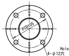
Figure from direction of A A矢視
